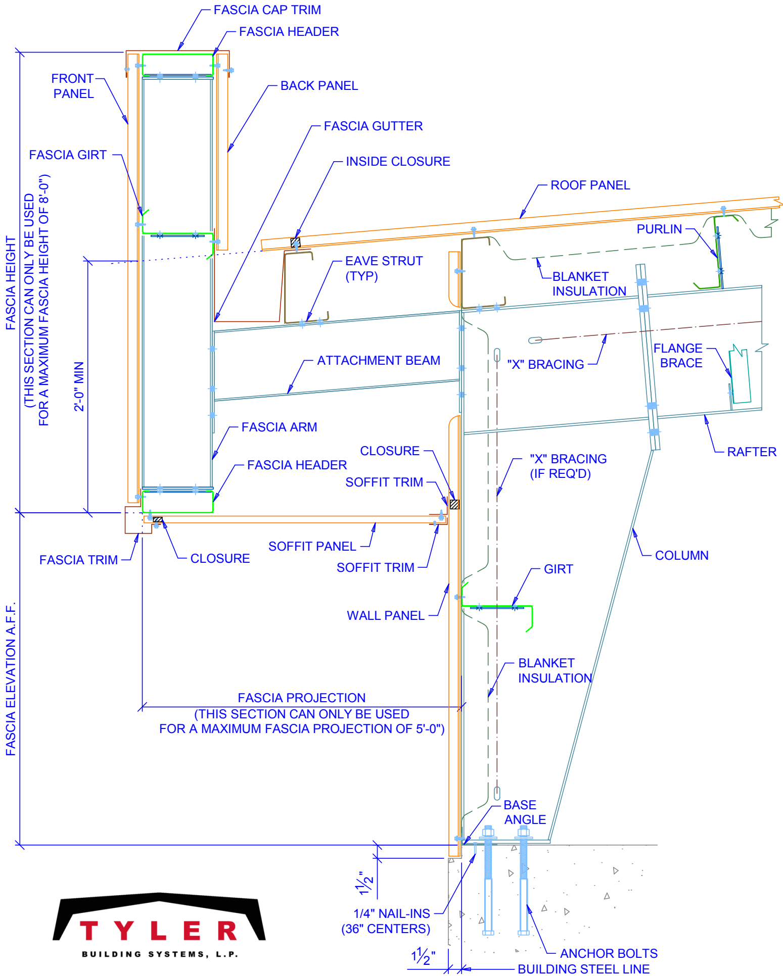
STANDARD FASCIA SECTION AT LOW SIDE EAVE (FLUSH GIRTS SYSTEM)
