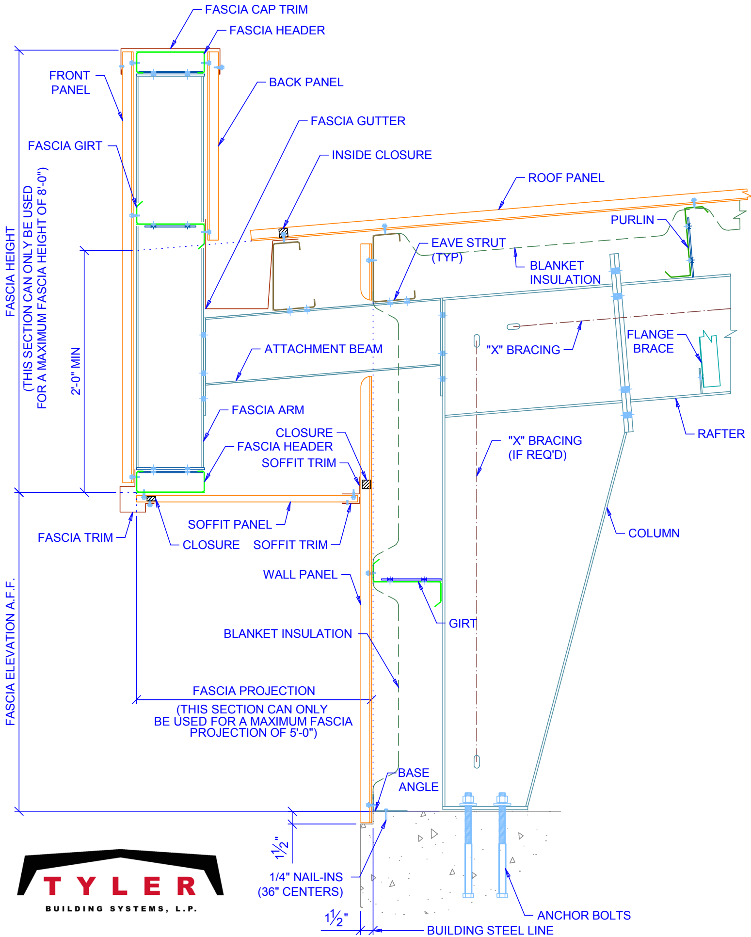
STANDARD FASCIA SECTION AT LOW SIDE EAVE (BYPASS GIRTS SYSTEM)
