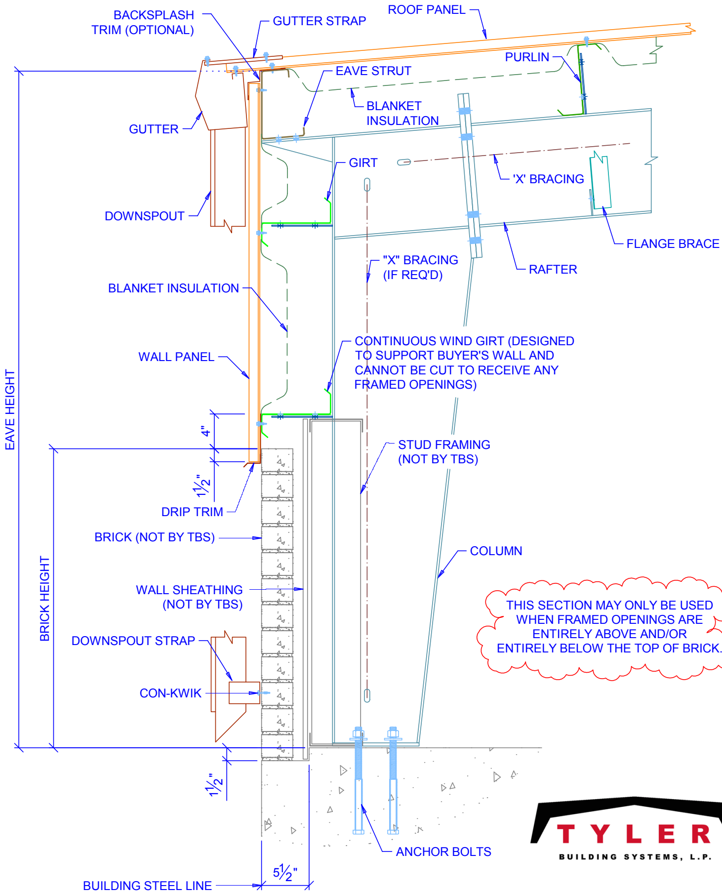
SIDEWALL SECTION AT PARTIAL BRICK WALL (BYPASS GIRT SYSTEM)
