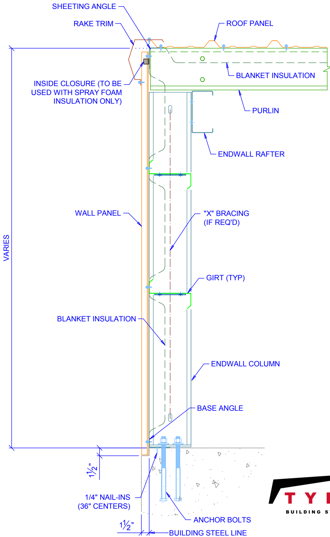
BEARING ENDWALL SECTION (FLUSH GIRT SYSTEM)
