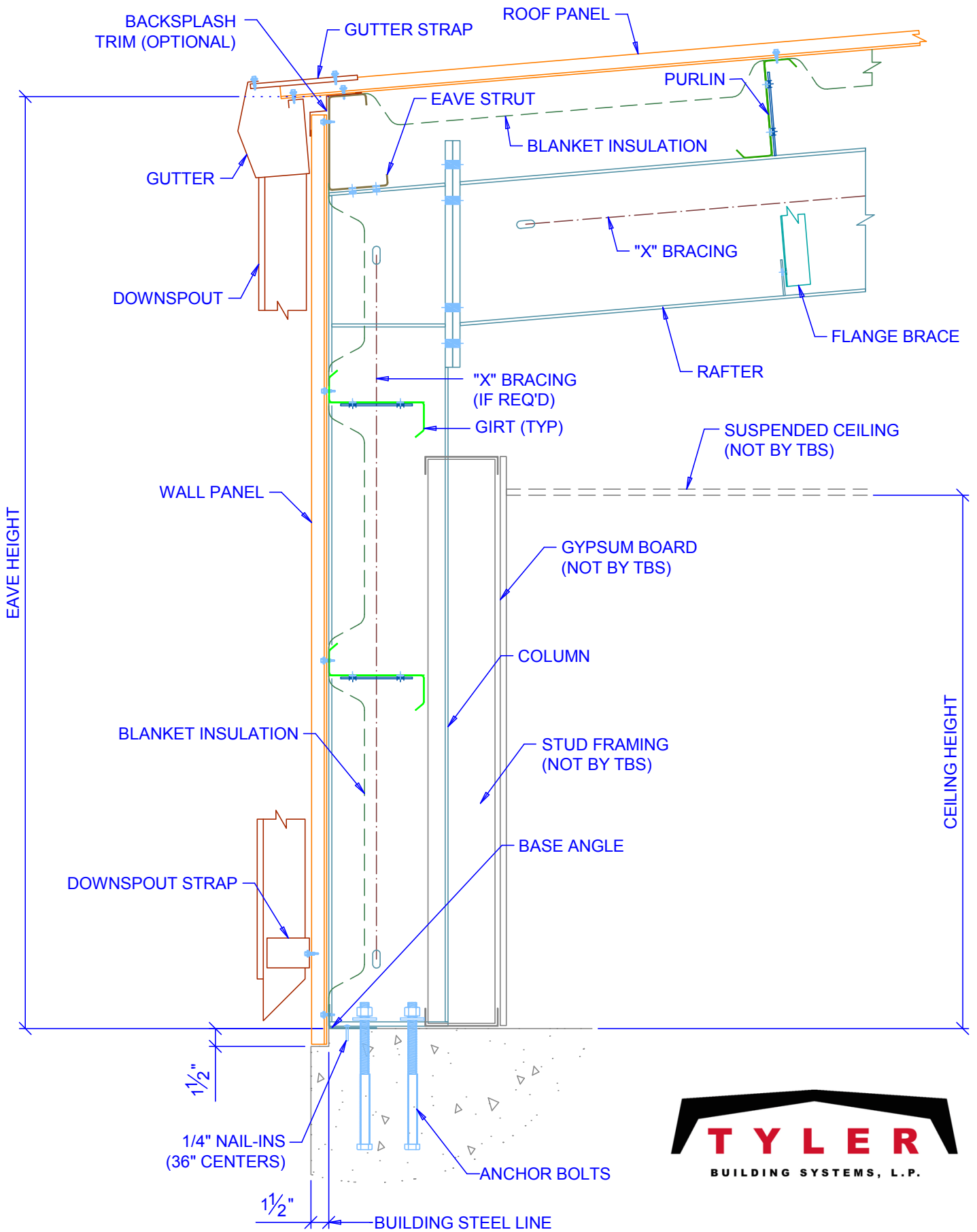
STANDARD SIDEWALL SECTION WITH STUD WALLS (FLUSH GIRTS SYSTEM)
