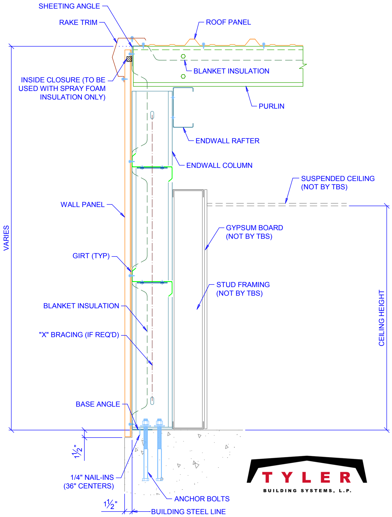
BEARING ENDWALL SECTION WITH STUD WALLS (FLUSH GIRT SYSTEM)
